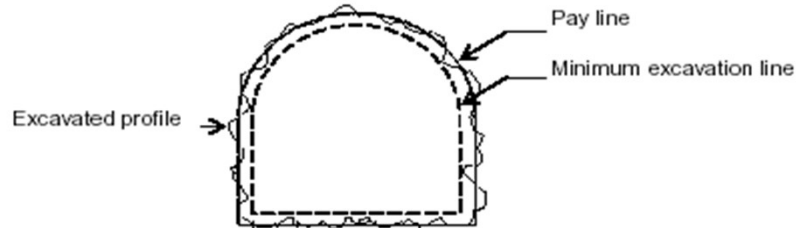
TYPICAL CROSS SECTION OF ADIT / TUNNEL
