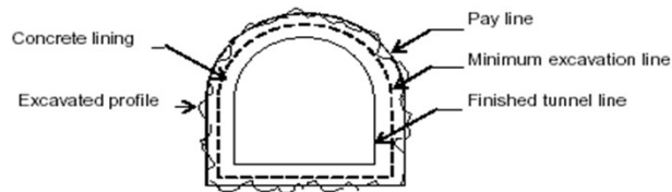
TYPICAL CROSS SECTION OF TUNNEL 4.50 m dia.
