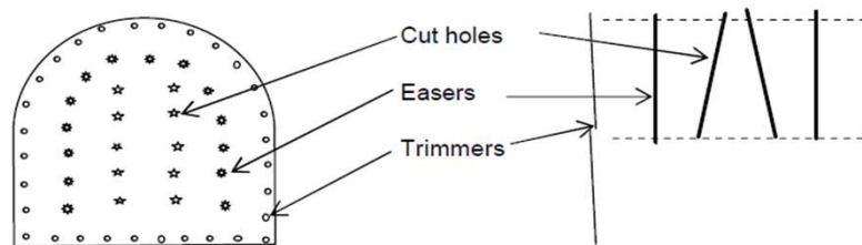
TYPICAL DRILLING PATTERN FOR ADIT / TUNNEL
